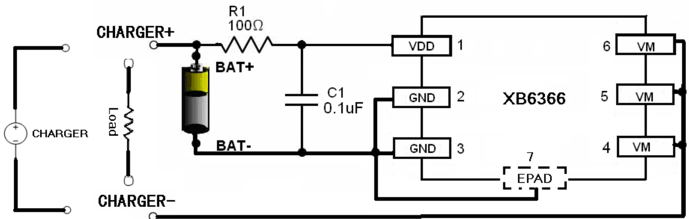
Fig 6 XB6366A in a Typical Battery Protection Circuit
